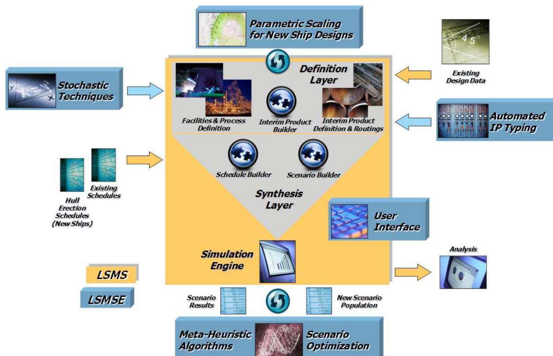
Figure 1: LSMSe Functional Diagram
