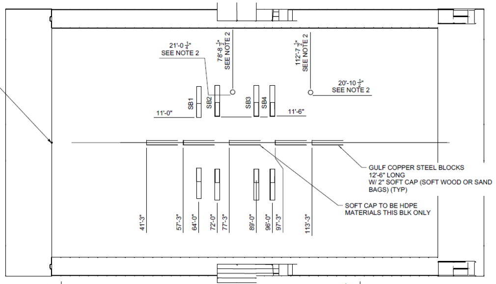
Figure 2: Docking 1 Blocking Plan
