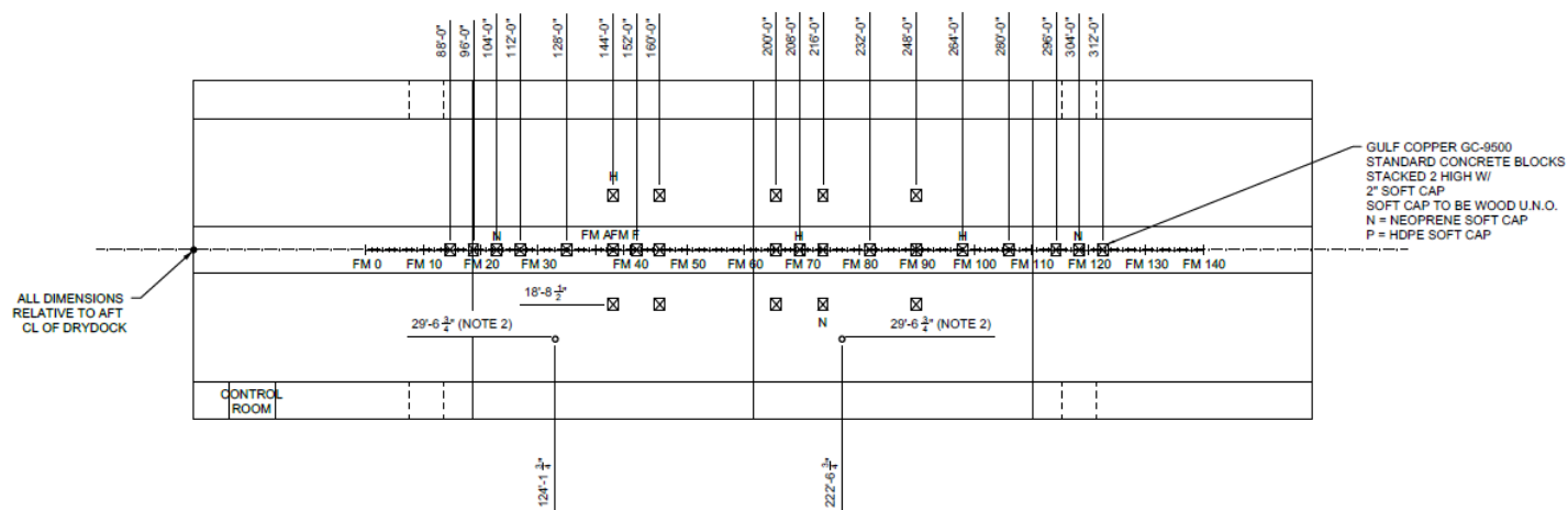
PLAN VIEW - BLOCKS
