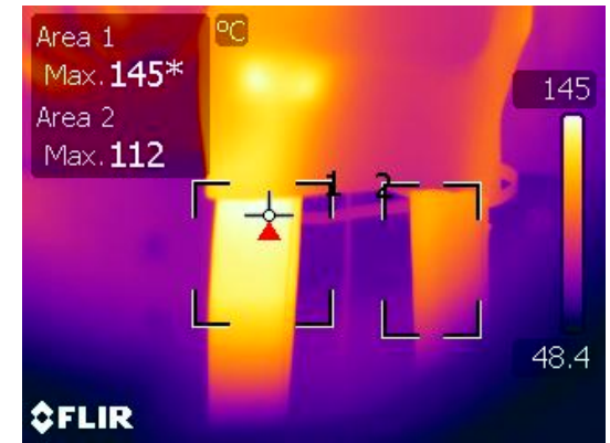
Thermal image of dust boot and cables with simulated fault
