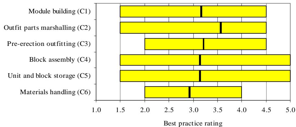
Figure 3.3 – Pre-erection activities
